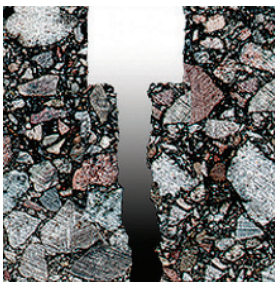
Routed Cracks increase crack seal longevity.
