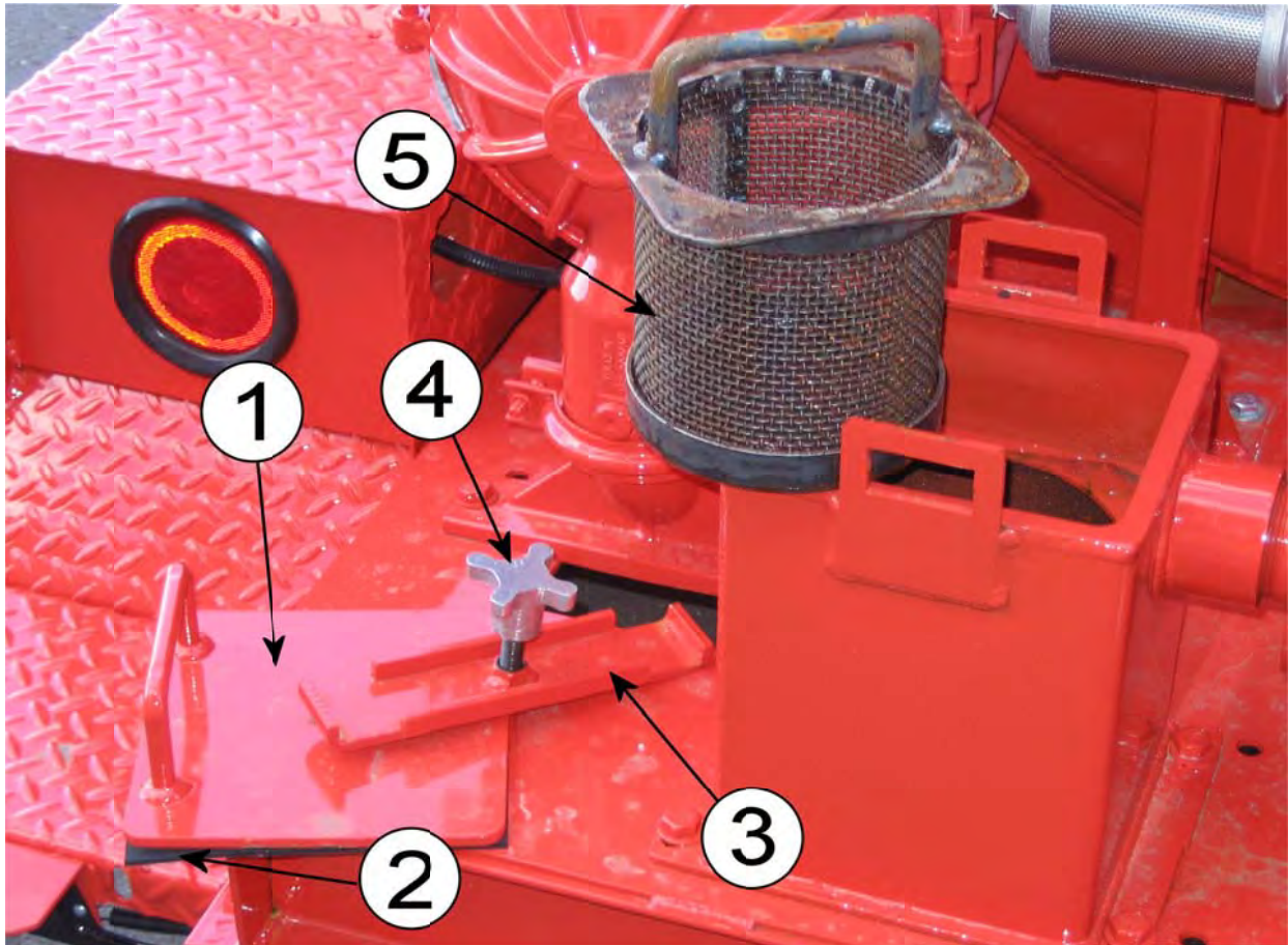
STRAINER BOX
